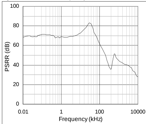
Figure 11. PSRR vs. Frequency; I_{out} = 10\text{mA}
