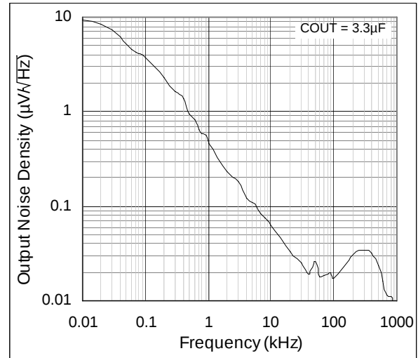
Figure 10. Spectral Noise vs. Freq.; I_{out} = 10\text{mA} ,
