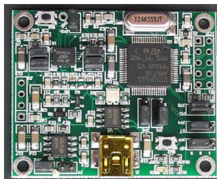
STEVAL-MKI077V1
