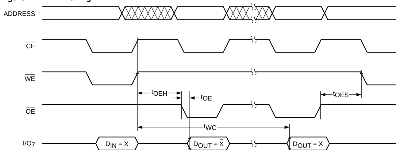
Figure 7. DATA Polling
