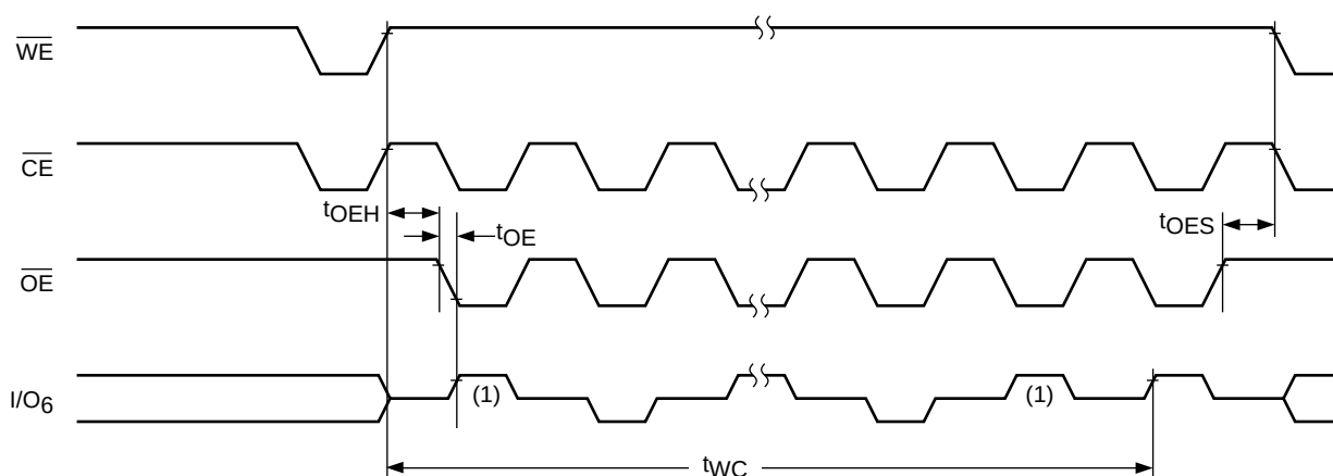
Figure 8. Toggle Bit
