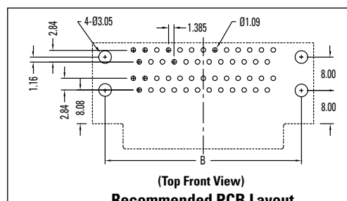
(Top Front View) Recommended PCB Layout
