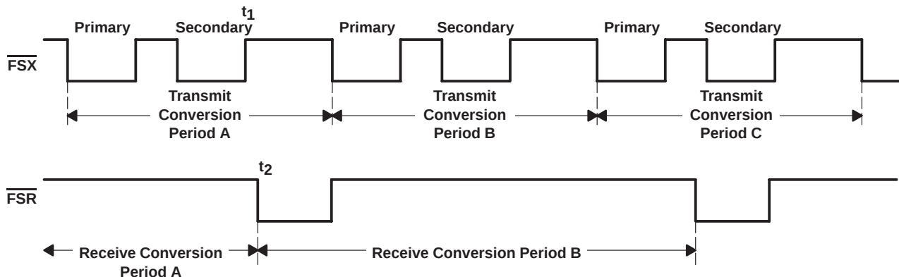
Figure 4. Receive and Transmit Periods for Primary and Secondary Data
