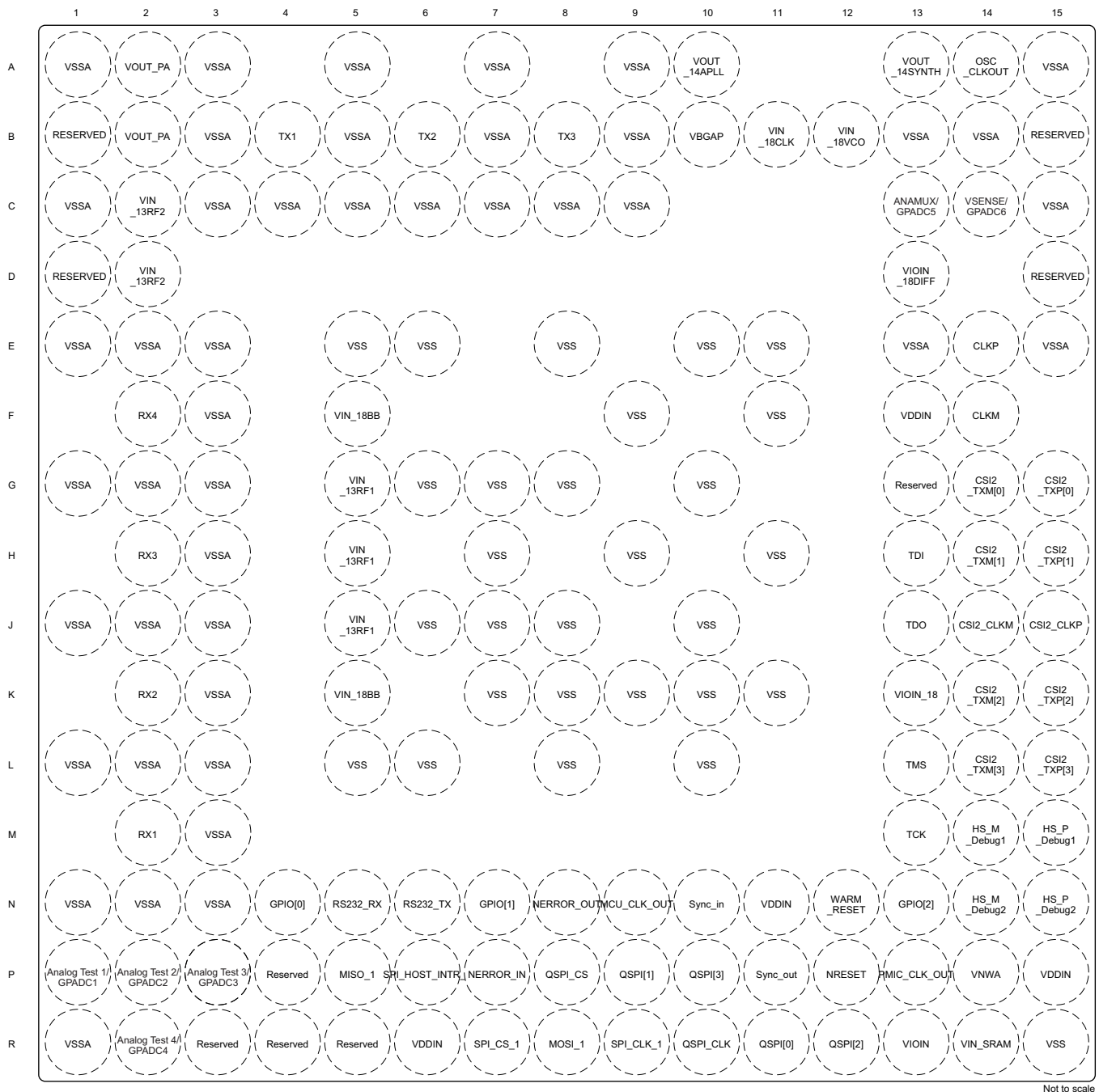
Figure 4-1. Pin Diagram
