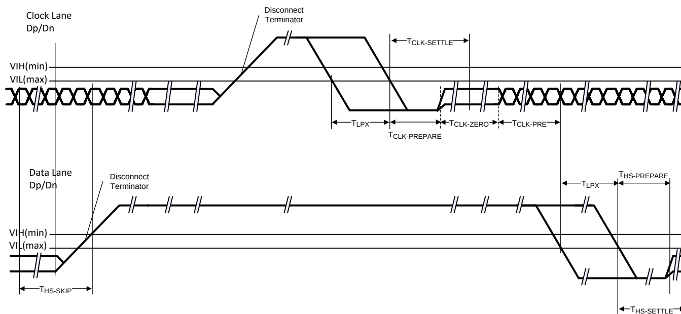
Figure 5-20. Switching the Clock Lane Between Clock Transmission and Low-Power Mode
