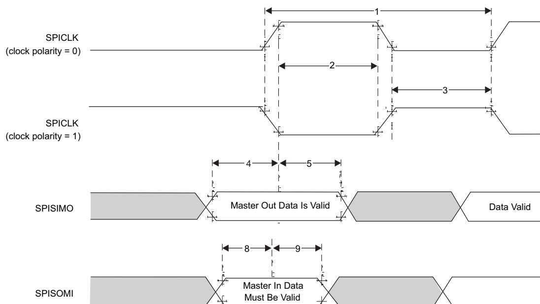
Figure 5-7. SPI Master Mode External Timing (CLOCK PHASE = 1)
