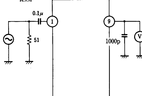
Test Circuit 10
