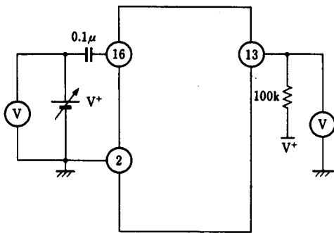
Test Cricuit 3
