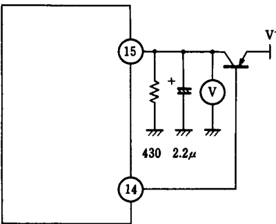
Test Circuit 8
