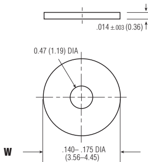
MGS/MGSD/MGSDD Mounting Pad
