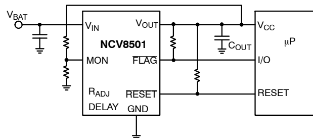
Figure 16. FLAG/Monitor Function
