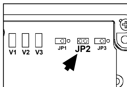
JP2 jumper ORRA receiver
