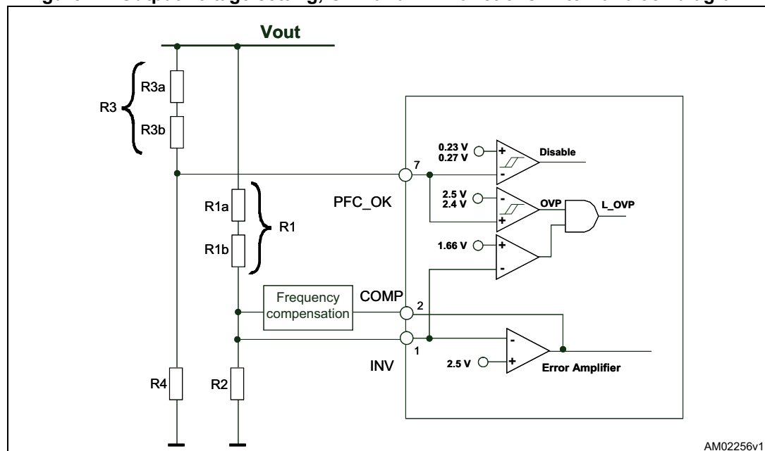
Figure 27. Output voltage setting, OVP and FFP functions: internal block diagram
