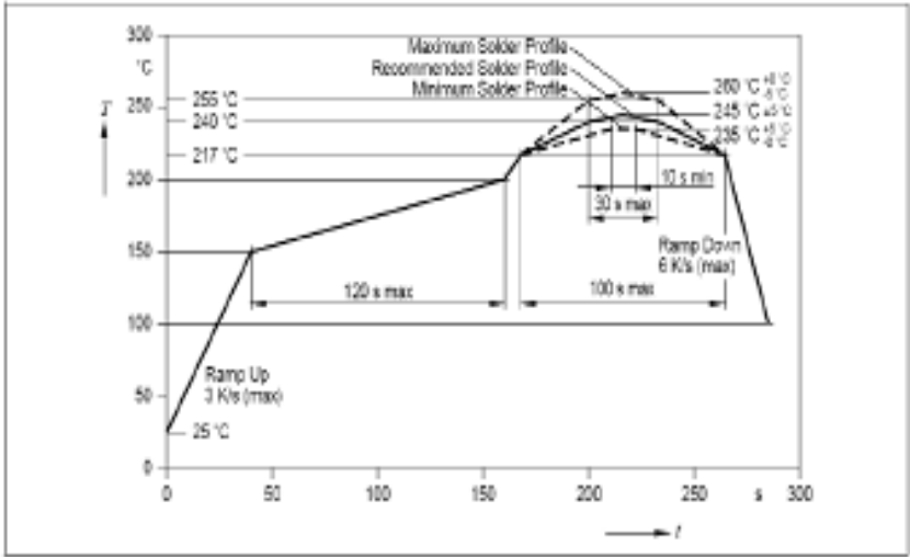
RoHS COMPLIANT SOLDER REFLOW PROFILE
