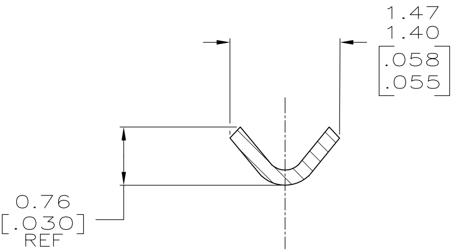
SECTION B-B SCALE 20:1
