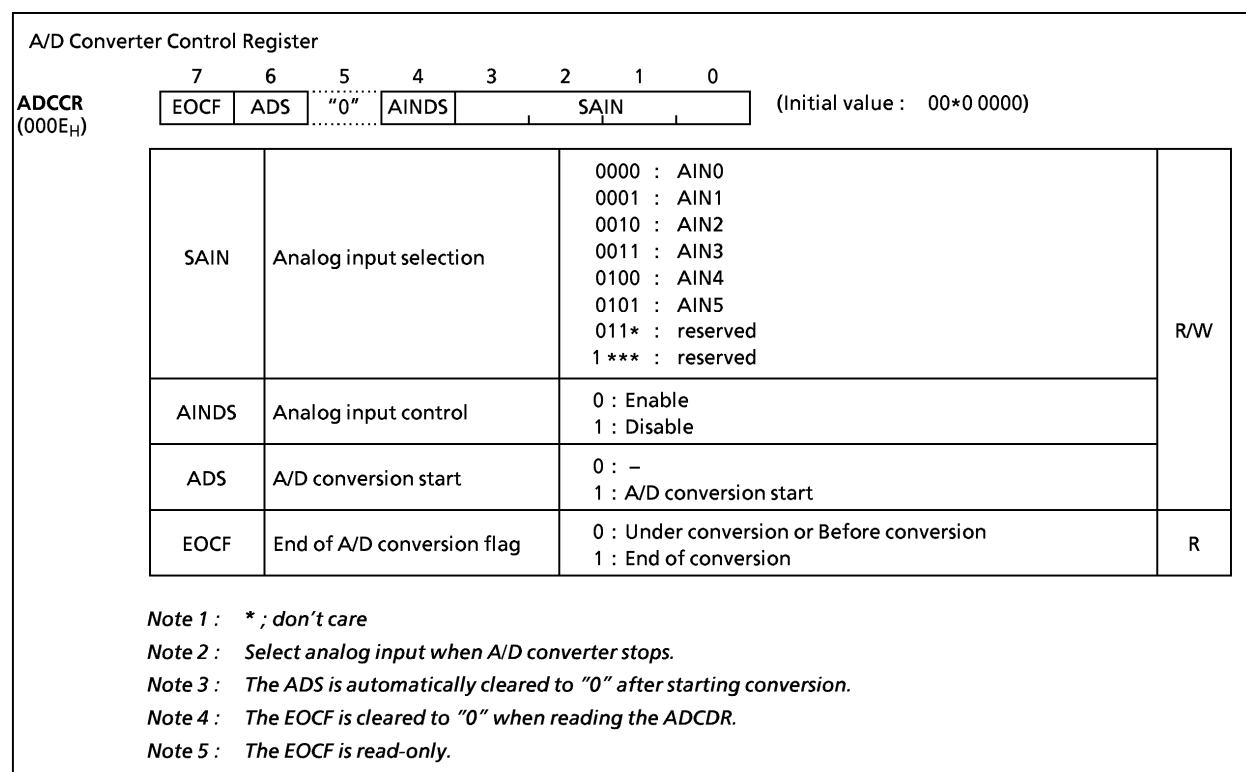
Figure 2-62. A/D converter control register
