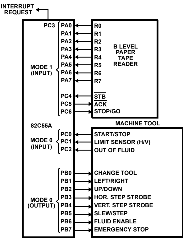
FIGURE 24. MACHINE TOOL CONTROLLER INTERFACE
