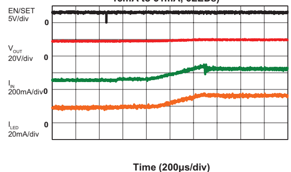
LED Current Transient ( V_{IN} = 3.6V , C_{IN} = 2.2\mu F , C_{OUT} = 2.2\mu F , R_{FB} = 8.3\Omega , S^2C data 16 to 1, 15mA to 31mA, 6 LEDs)
