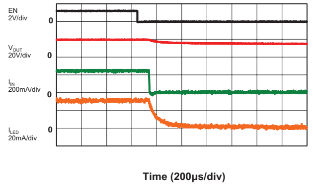
Turn Off ( V_{IN} = 3.6V , C_{IN} = 2.2\mu F , C_{OUT} = 2.2\mu F , R_{FB} = 8.3\Omega , 6 LEDs)
