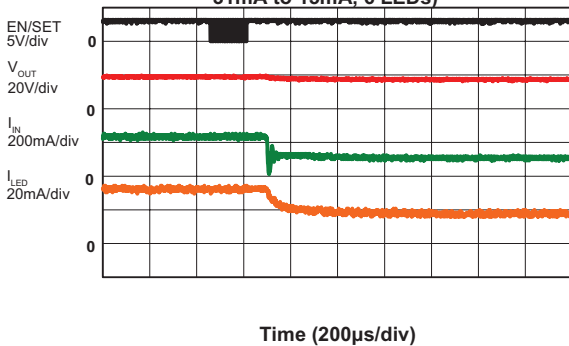
LED Current Transient ( V_{IN} = 3.6V , C_{IN} = 2.2\mu F , C_{OUT} = 2.2\mu F , R_{FB} = 8.3\Omega , S^2C data 1 to 16, 31mA to 15mA, 6 LEDs)
