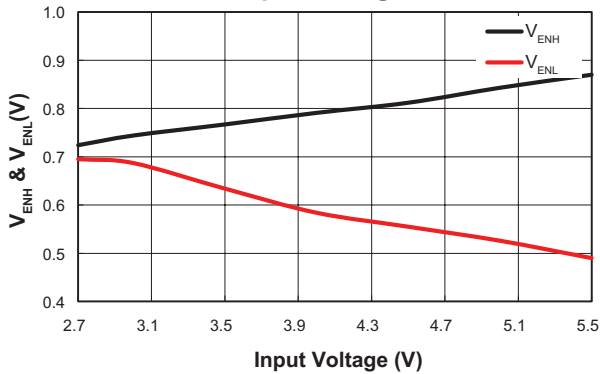
EN Input High/Low Threshold Voltage vs Input Voltage
