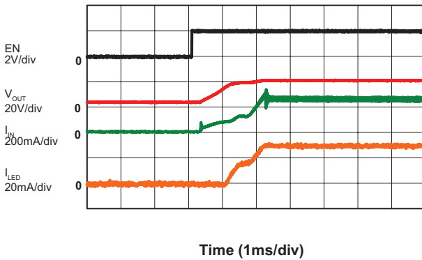
Start Up Waveform ( V_{IN} = 3.6V , C_{IN} = 2.2\mu F , C_{OUT} = 2.2\mu F , R_{FB} = 8.3\Omega , 6 LEDs)
