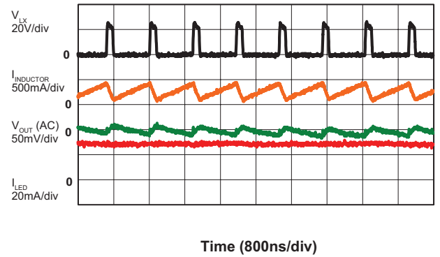
Operation Waveform ( V_{IN} = 3.6V , C_{IN} = 4.7\mu F , C_{OUT} = 2.2\mu F , R_{FB} = 8.3\Omega , 6 LEDs)
