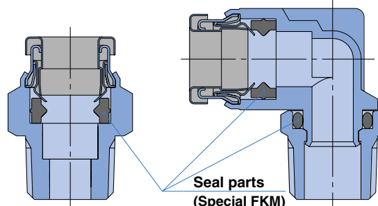
Male connector
