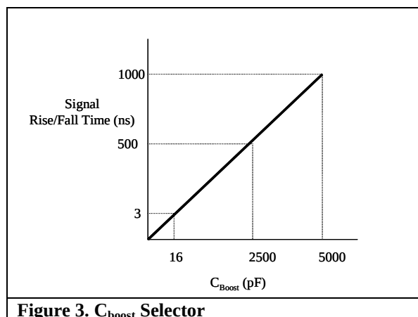
Figure 3. C_{boost} Selector
