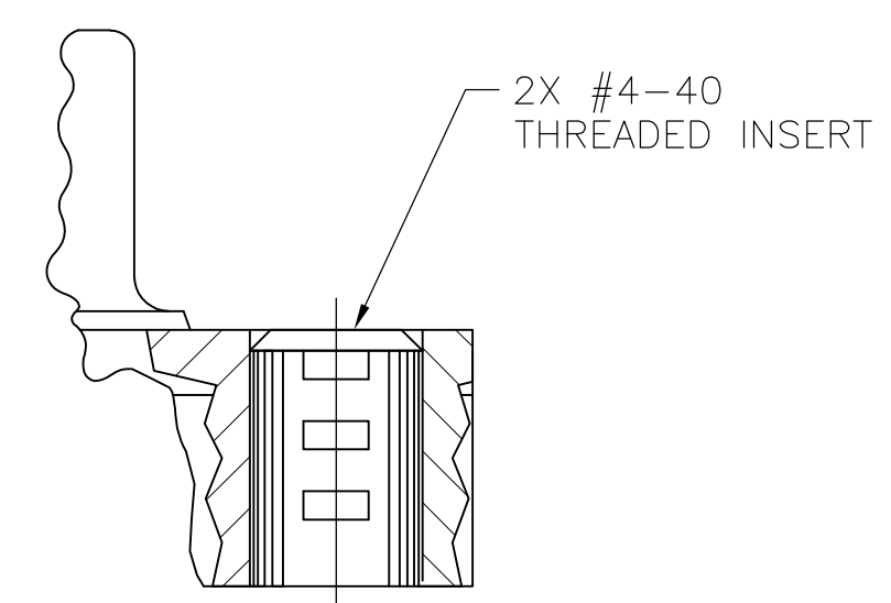
DETAIL B
