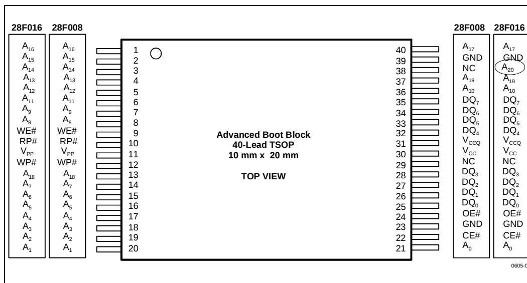
Figure 1. 40-Lead TSOP Package
