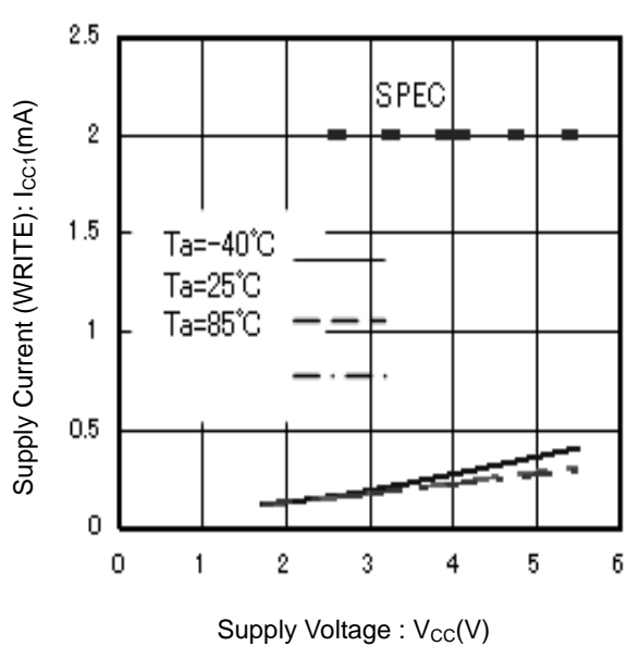
Figure 9. Supply Current (WRITE) vs Supply Voltage (f SCL =400kHz)
