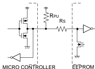
Figure 46. I/O Circuit
