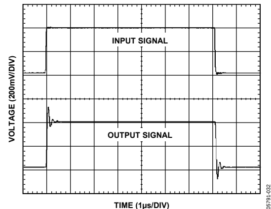
Figure 31. Capacitive Load Drive Without Snubber Network
