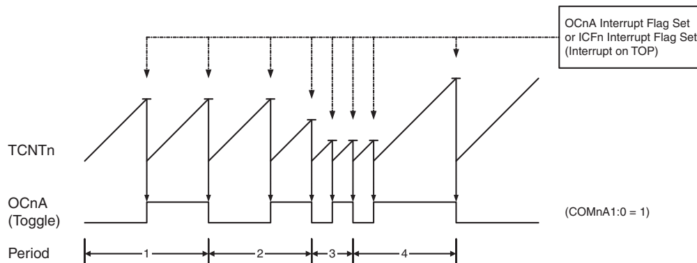
Figure 4-42. CTC Mode, Timing Diagram
