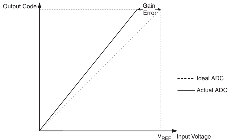
Figure 4-68. Gain Error
