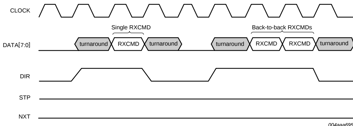
Fig 10. Single and back-to-back RXCMDs from the ISP1507 to the link
