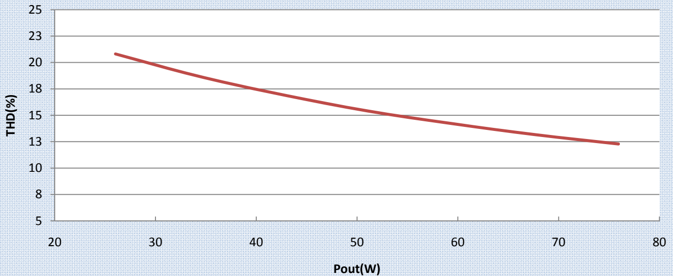
THD VS Pout @ TC 80C @ Vin-230V
