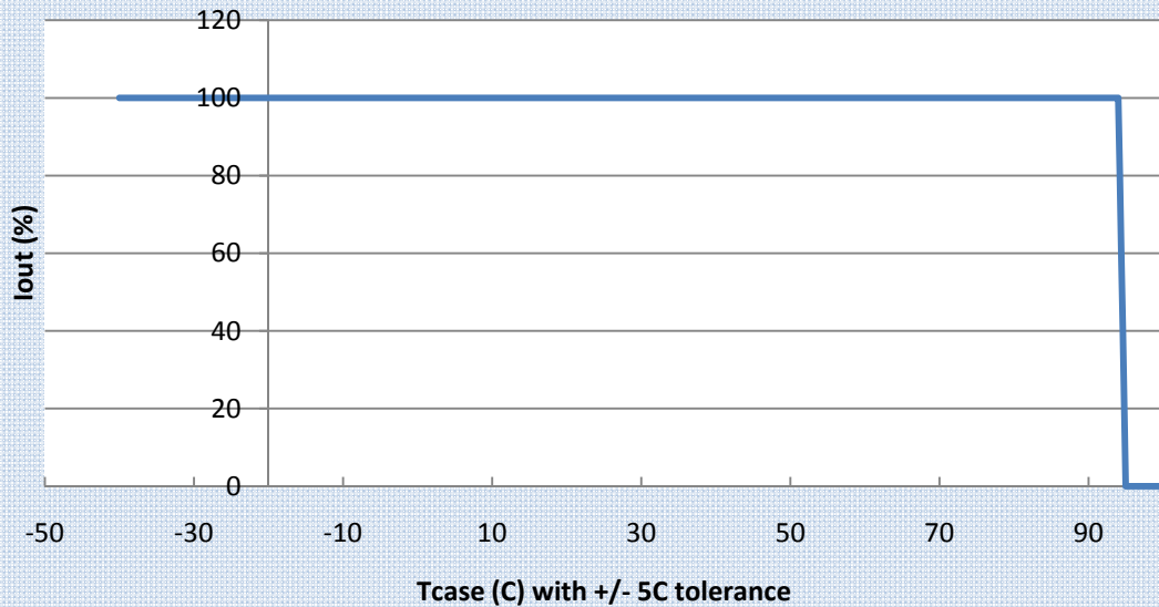
I out (%) VS T case
