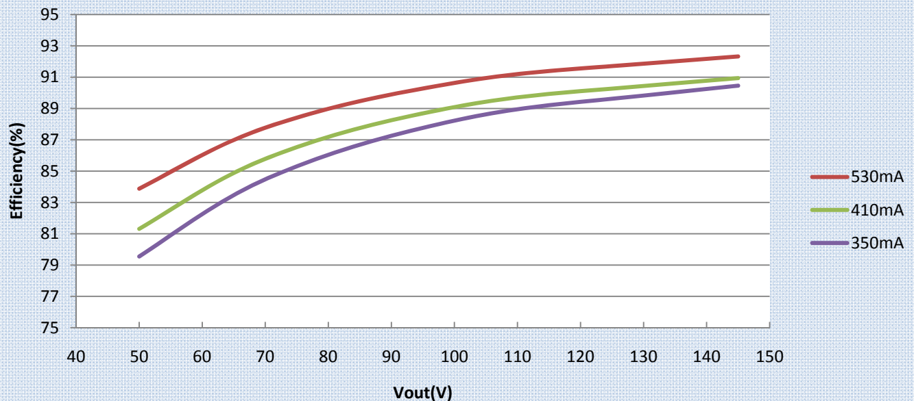
Efficiency VS Vout @ TC 80C @ Vin-230V
