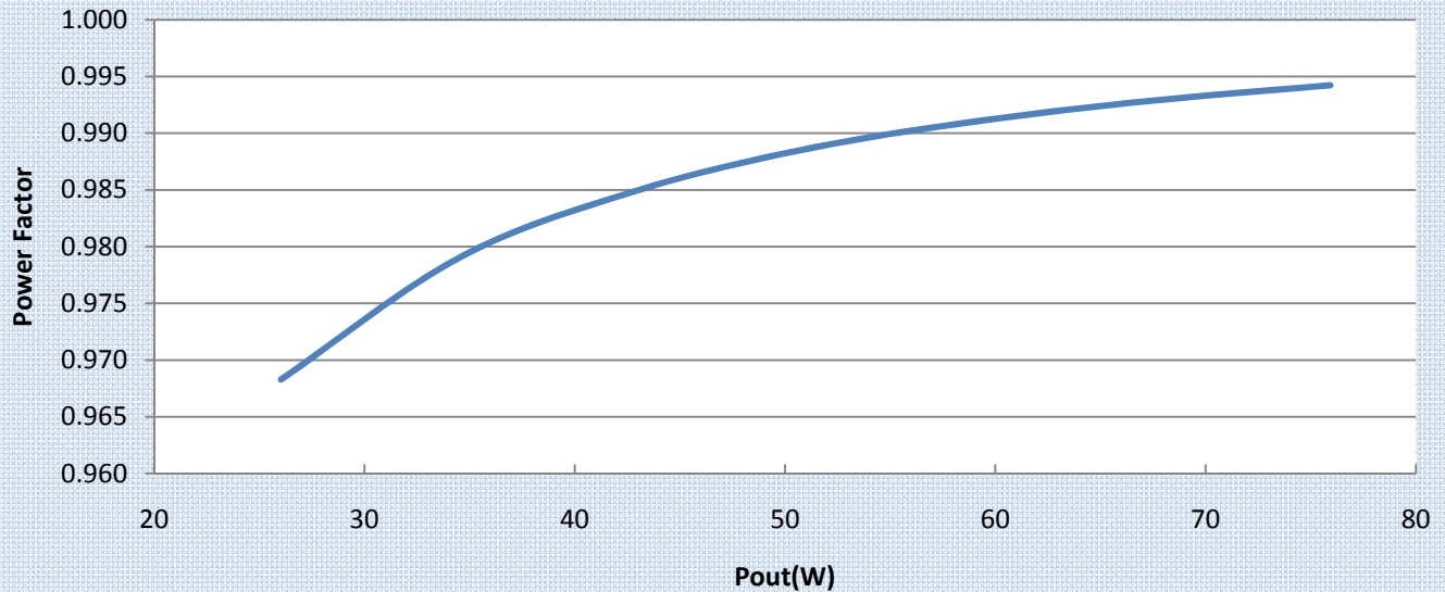
pf VS Pout @ TC 80C @ Vin-230V
