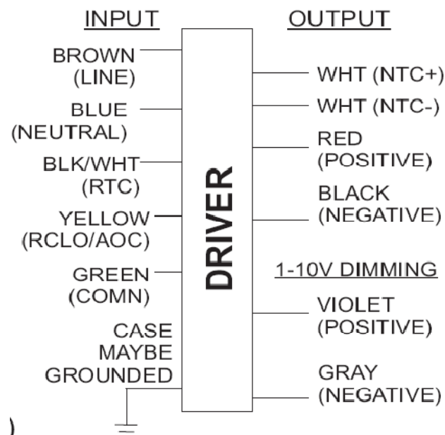
Wire Diagram
