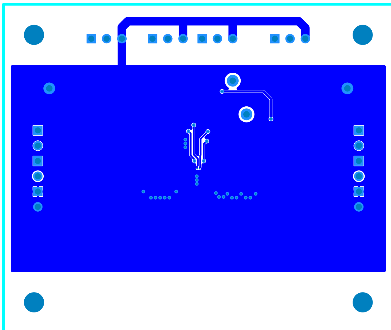
Figure 4. Bottom Layer Routing
