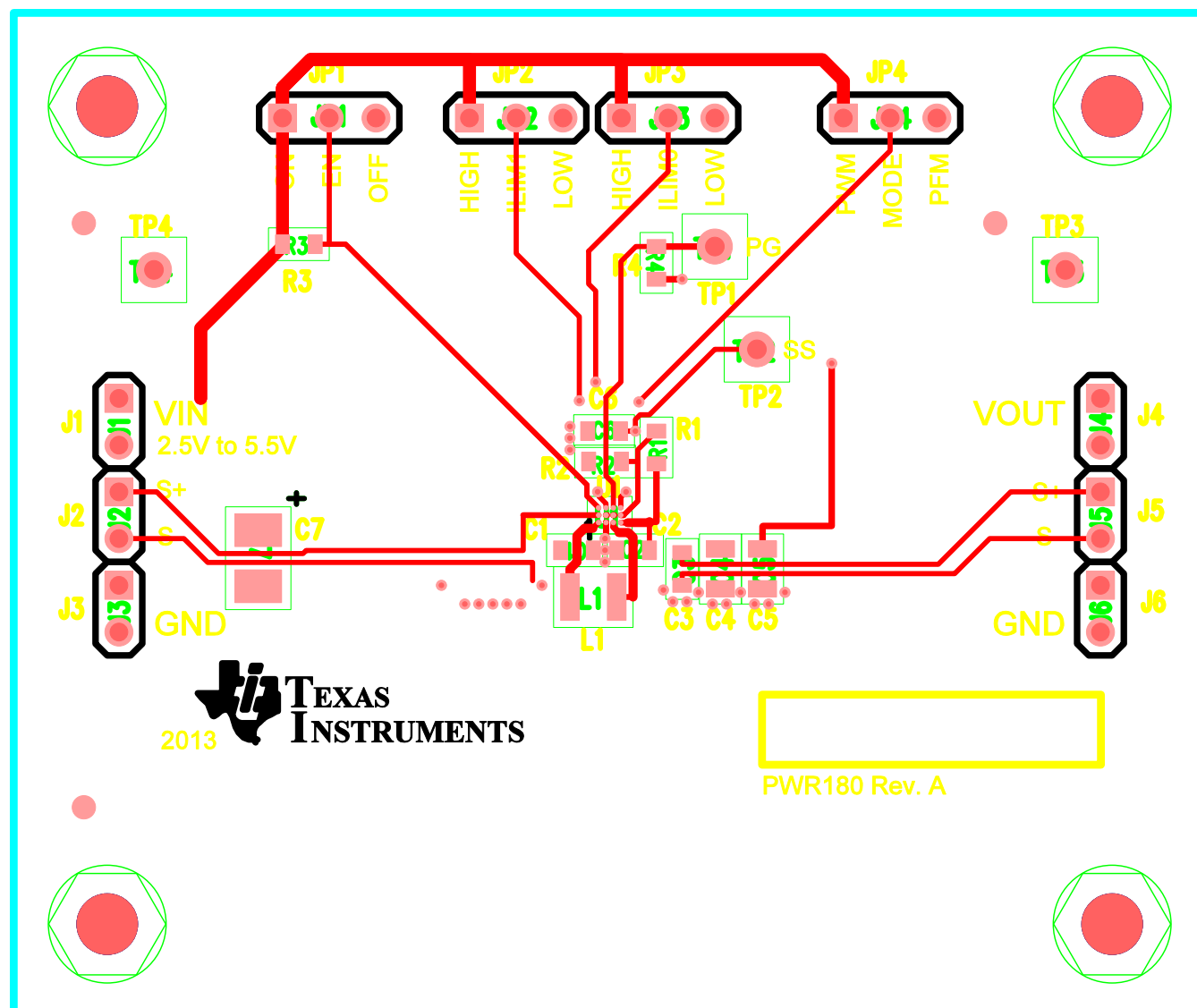
Figure 2. Assembly Layer
