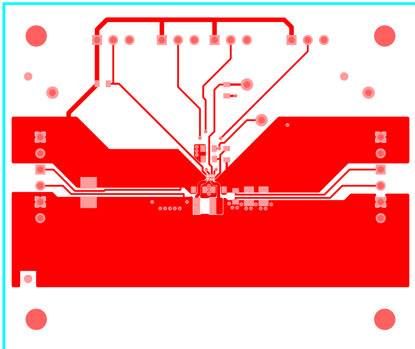
Figure 3. Top Layer Routing
