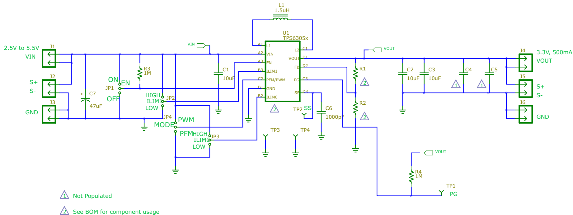
Figure 5. TPS6305xEVM-180 Schematic
