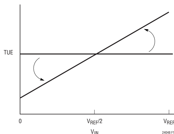
Figure 13. Offset/Full-Scale Shift
