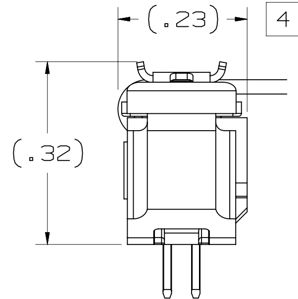
VERTICAL ASSEMBLY
