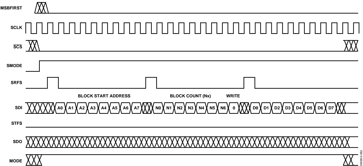
Figure 53. SPORT Write MSB_FIRST = 0
