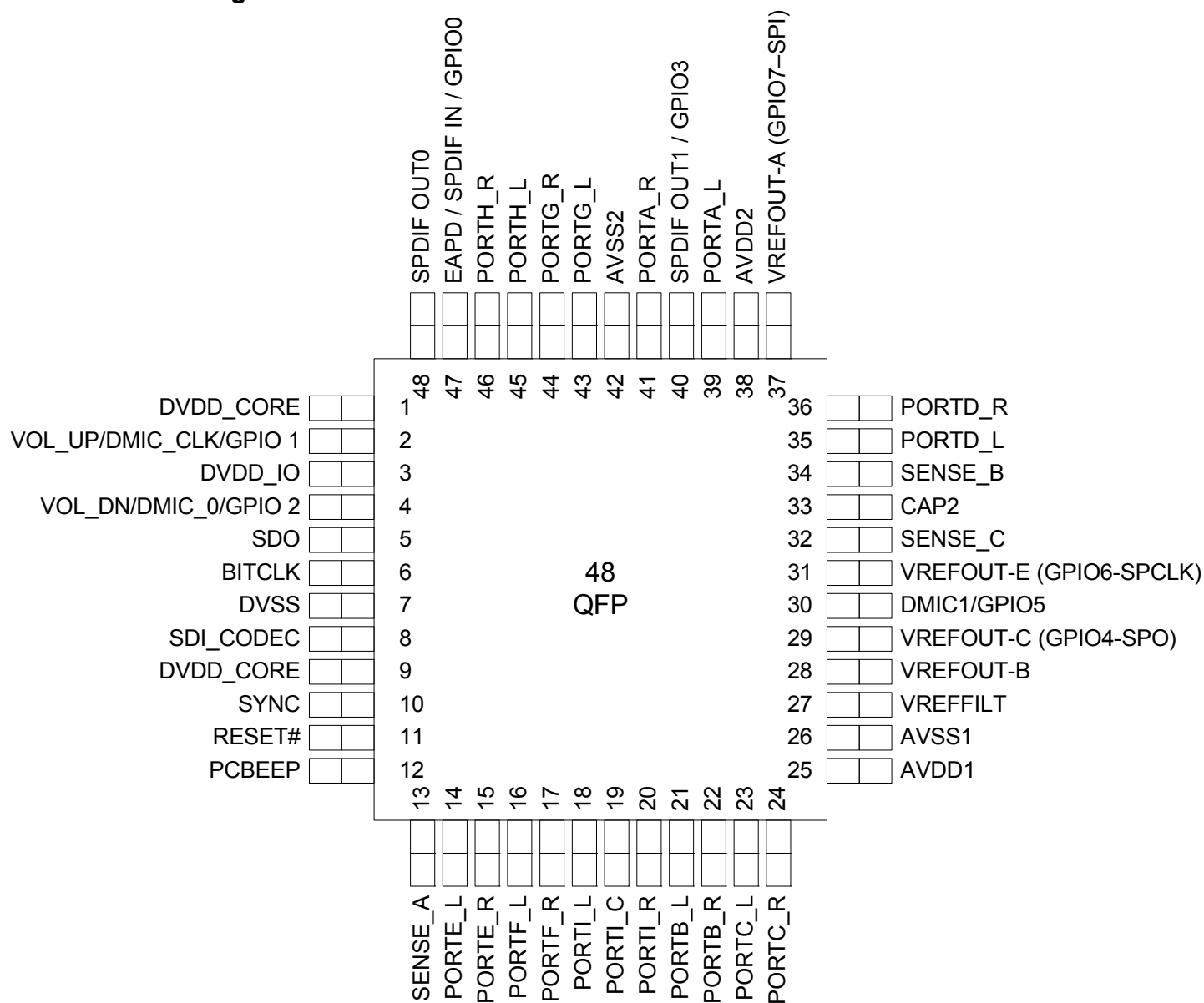
Figure 13. Pin Assignment
