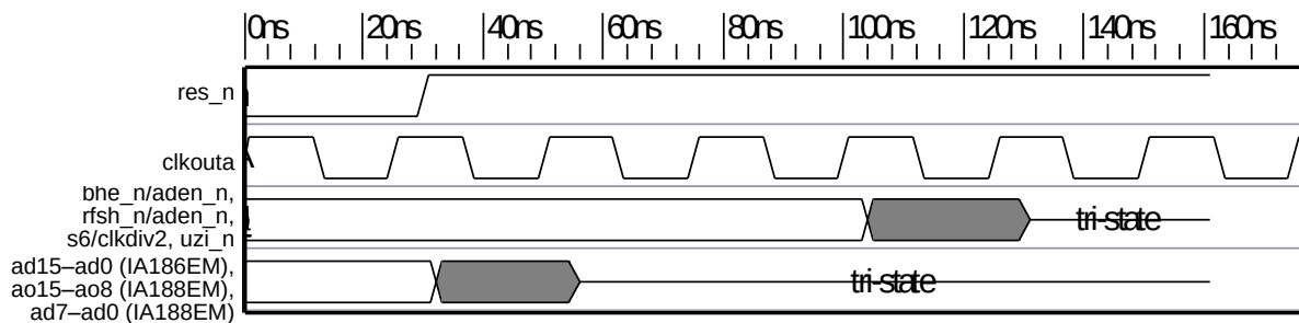
Figure 26. Reset 2
