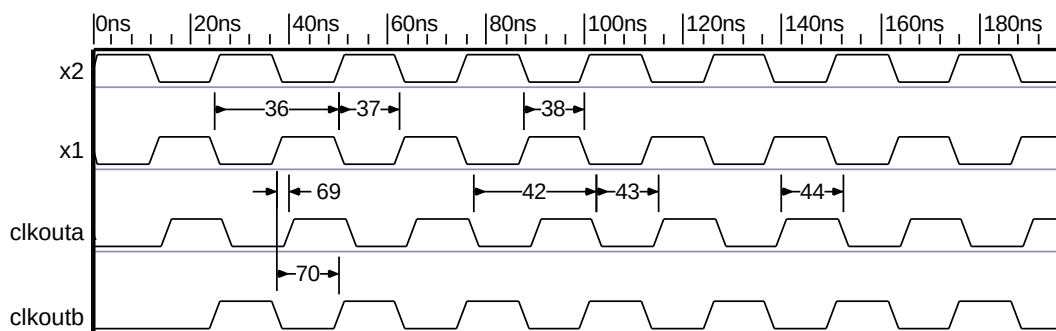
Figure 20. Clock—Active Mode
