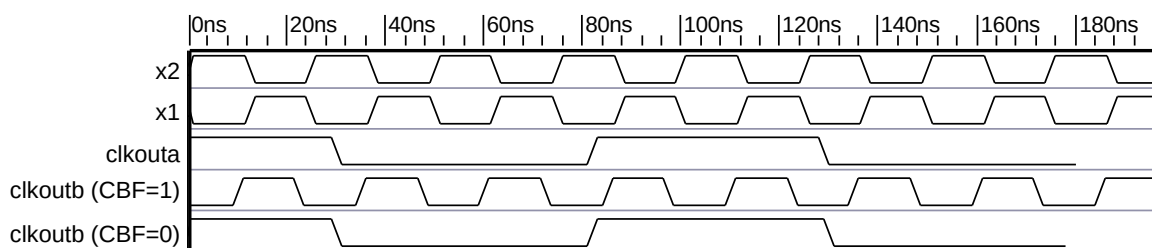
Figure 21. Clock—Power-Save Mode
