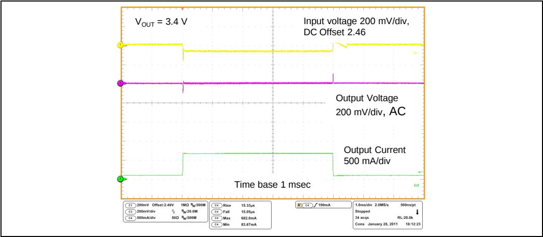
Figure 14. V_{IN} = 2.4 V , V_{OUT} = 3.4 V , I_{OUT} = from 80 mA to 630 mA
