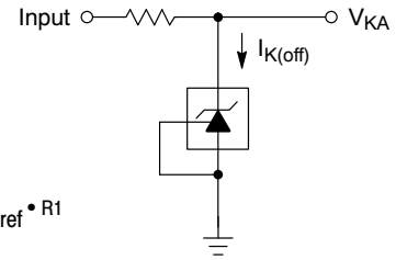
Figure 5. Test Circuit for I_{K(off)}
