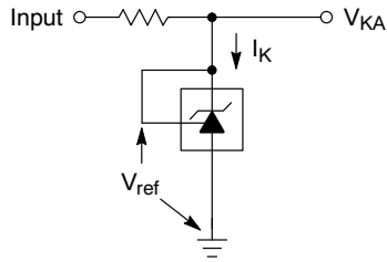
Figure 3. Test Circuit for V_{KA} = V_{ref}
