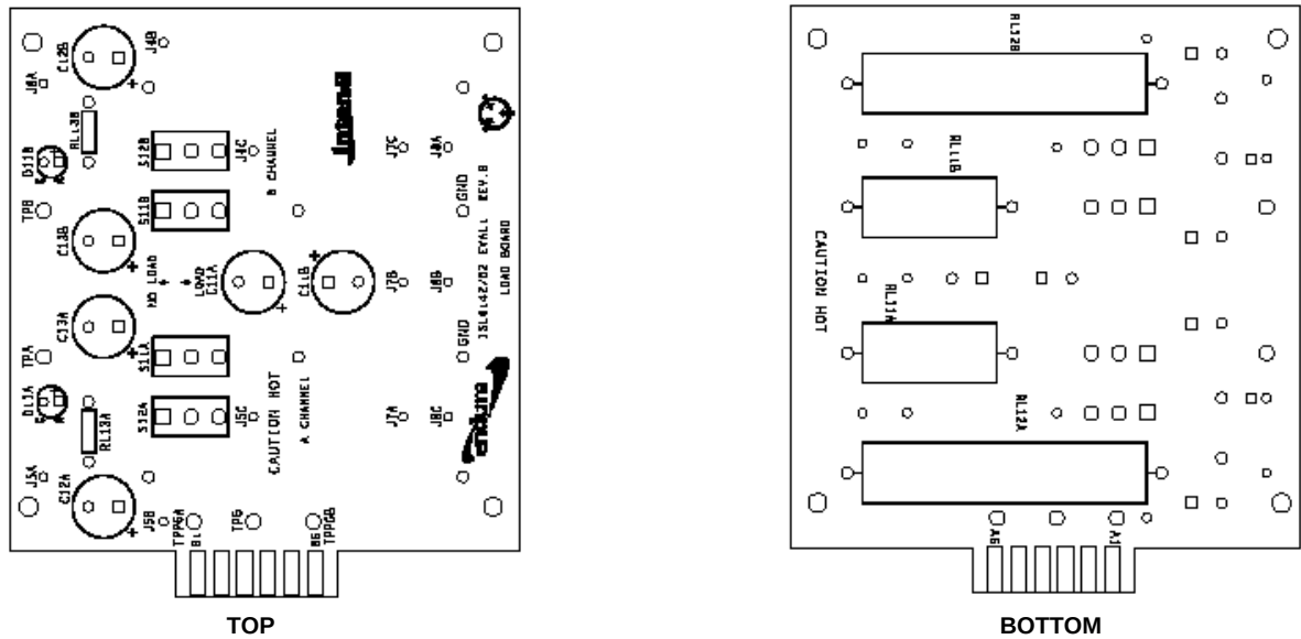
FIGURE 9. LOAD BOARD
