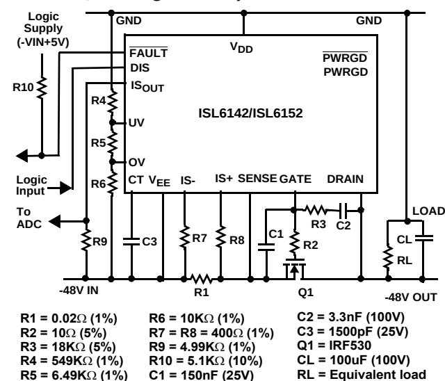
FIGURE 4. TYPICAL APPLICATION
