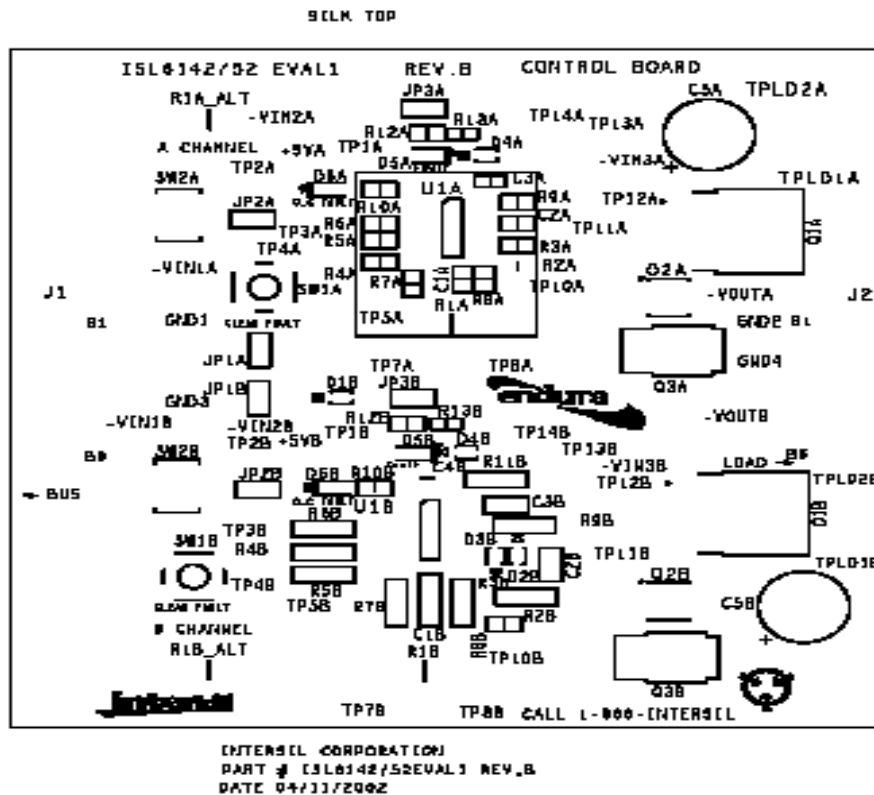
FIGURE 10. CONTROL BOARD
