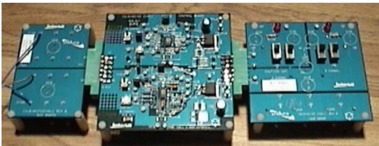
BUS BOARD
