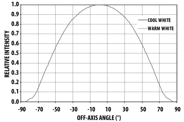
Figure 4. Radiation Pattern
