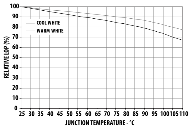
Figure 8. Relative LOP vs. junction temperature
