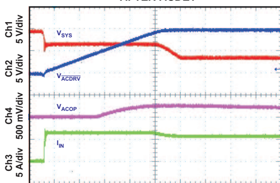
SELECTOR GATE DRIVE VOLTAGES, 700 MS DELAY AFTER ACDET
