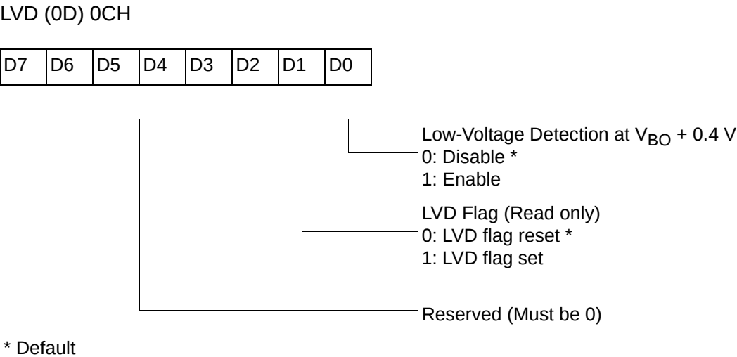
Figure 38. Low-Voltage Detection
