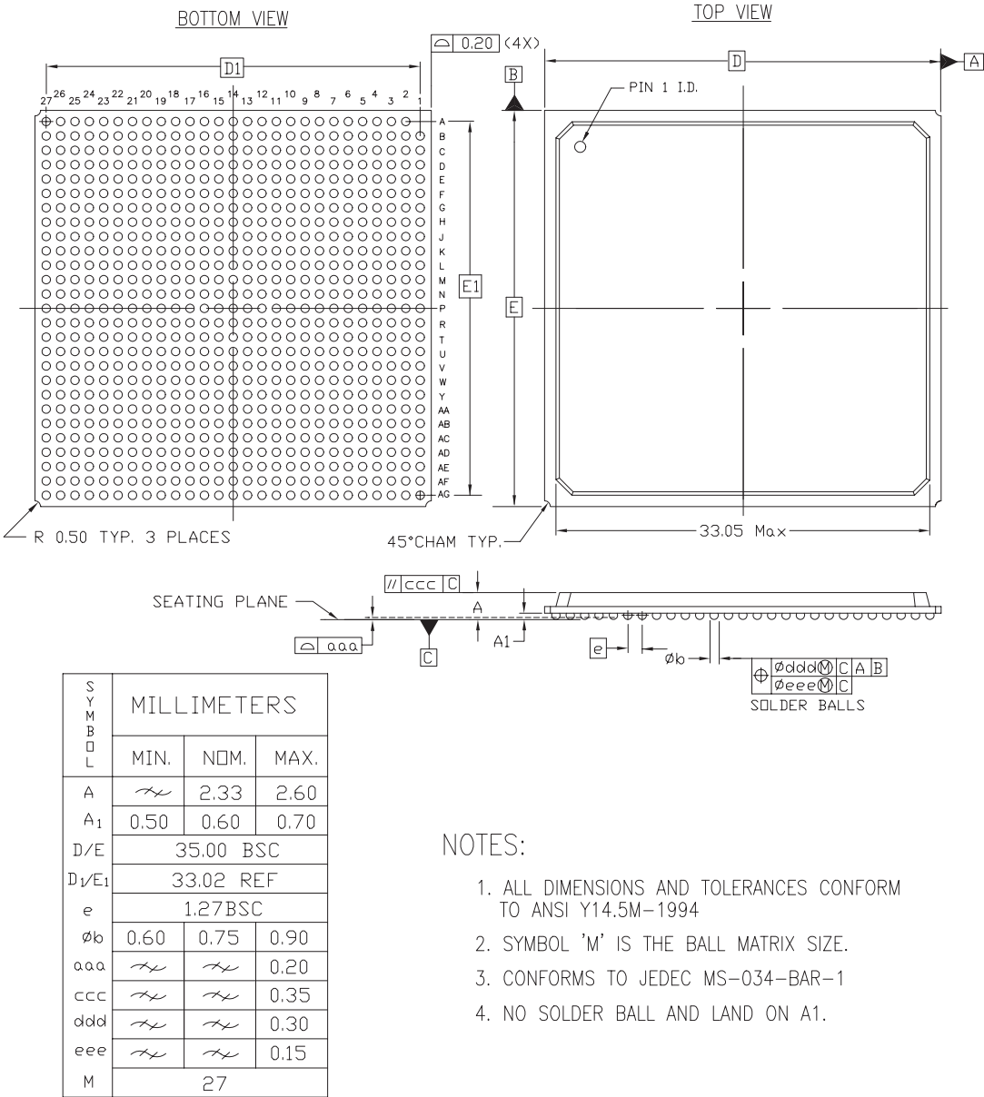
Figure 54: BG728 Standard BGA Package Specifications
