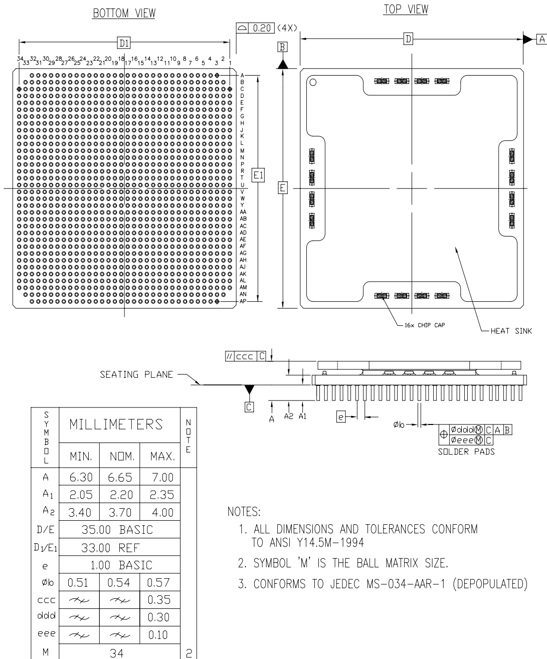
Figure 56: CF1144 Ceramic Flip-Chip Fine-Pitch CGA Package Specifications
