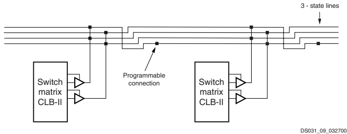
Figure 29: 3-State Buffer Connection to Horizontal Lines
