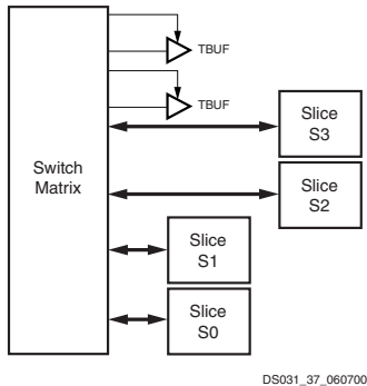
Figure 28: Virtex-II 3-State Buffers
