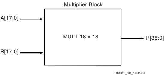
Figure 37: Multiplier Block
