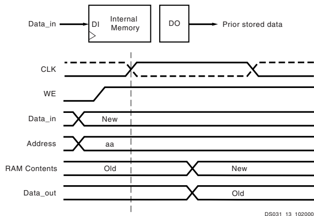
Figure 33: READ_FIRST Mode
