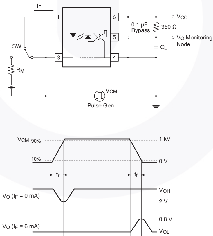
Figure 16. Test Circuit for Instantaneous Common-Mode Rejection Voltage
