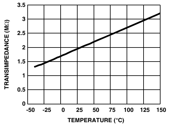
FIGURE 48. TRANSIMPEDANCE vs TEMPERATURE
