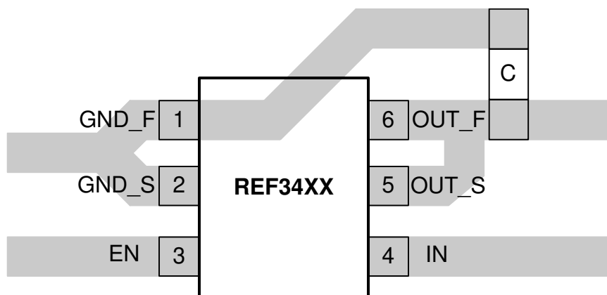
Figure 12-1. REF34xx Layout Example
