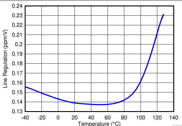
Figure 7-6. Line Regulation
