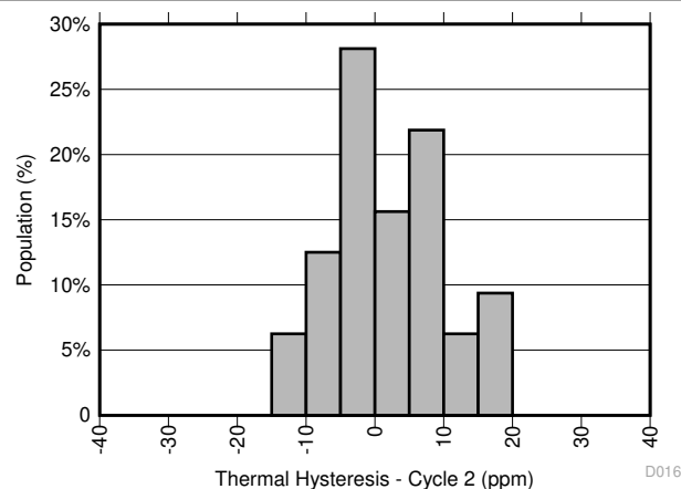
Figure 7-18. Thermal Hysteresis Distribution (Cycle 2)
