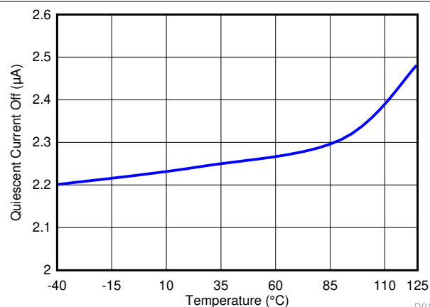
Figure 7-16. Quiescent Current Shutdown Mode
