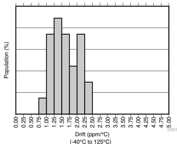
Figure 7-1. Temperature Drift
