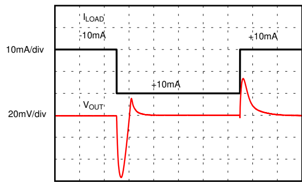
Figure 7-13. Load Transient
