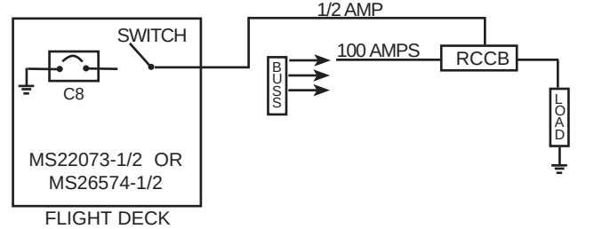
Distributed Load Concept
