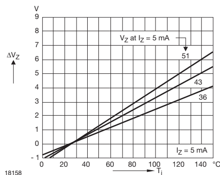
Fig. 11 - Change of Zener Voltage vs. Junction Temperature
