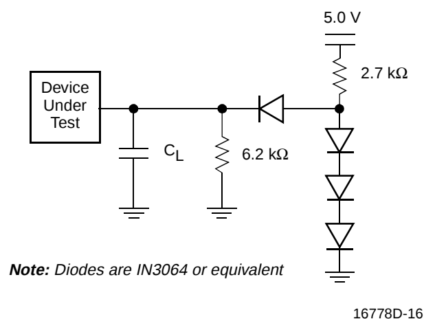
Figure 8. Test Setup
