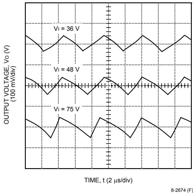
Figure 6. Typical HW050AF1 Output Ripple Voltage 3.3 V Output at Room Temperature and I_o = I_{o, \text{max}} , Different Input Voltage
