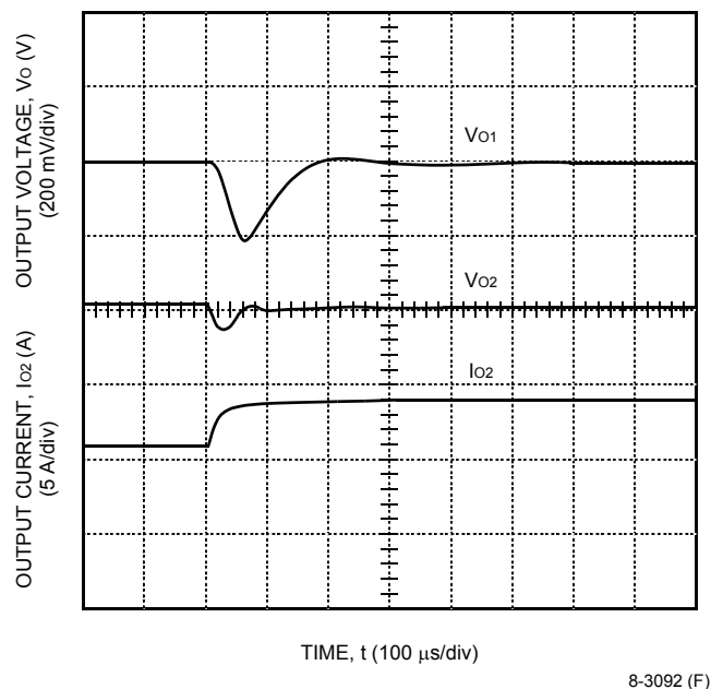
Figure 16. Typical HW050FG1 Transient Response to Step Increase in Load, I_{O2} = 50\% to 75\% of I_{O2, \text{max}} , I_{O1} = 30\% of I_{O1, \text{max}} , at Room Temperature and 48 V Input (Waveform Averaged to Eliminate Ripple Component.)
