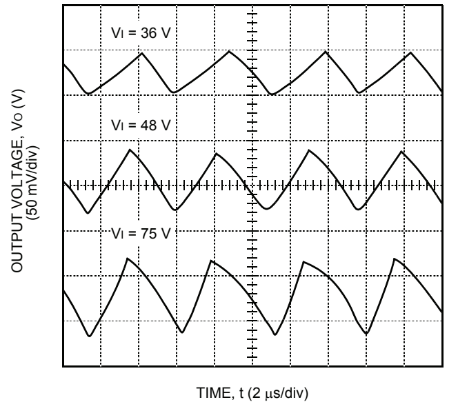
Figure 7. Typical HW050FG1 Output Ripple Voltage 3.3 V Output at Room Temperature and I_o = I_{o, \text{max}} , Different Input Voltage
