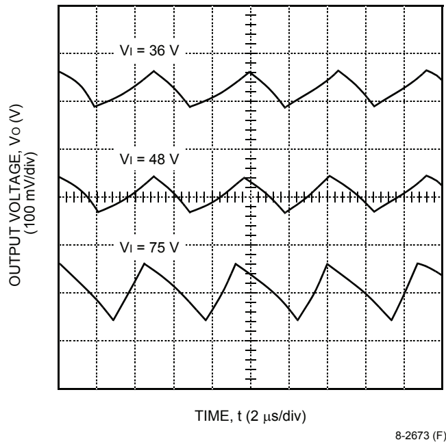
Figure 5. Typical HW050AF1 Output Ripple Voltage 5 V Output at Room Temperature and I_o = I_{o, \text{max}} , Different Input Voltage
