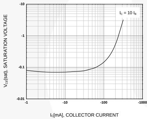
Figure 3. Collector-Emmitter Saturation Voltage
