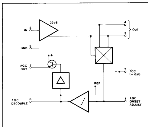
Fig. 2 Block diagram
