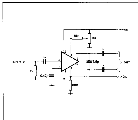
Fig. 3 Test circuit
