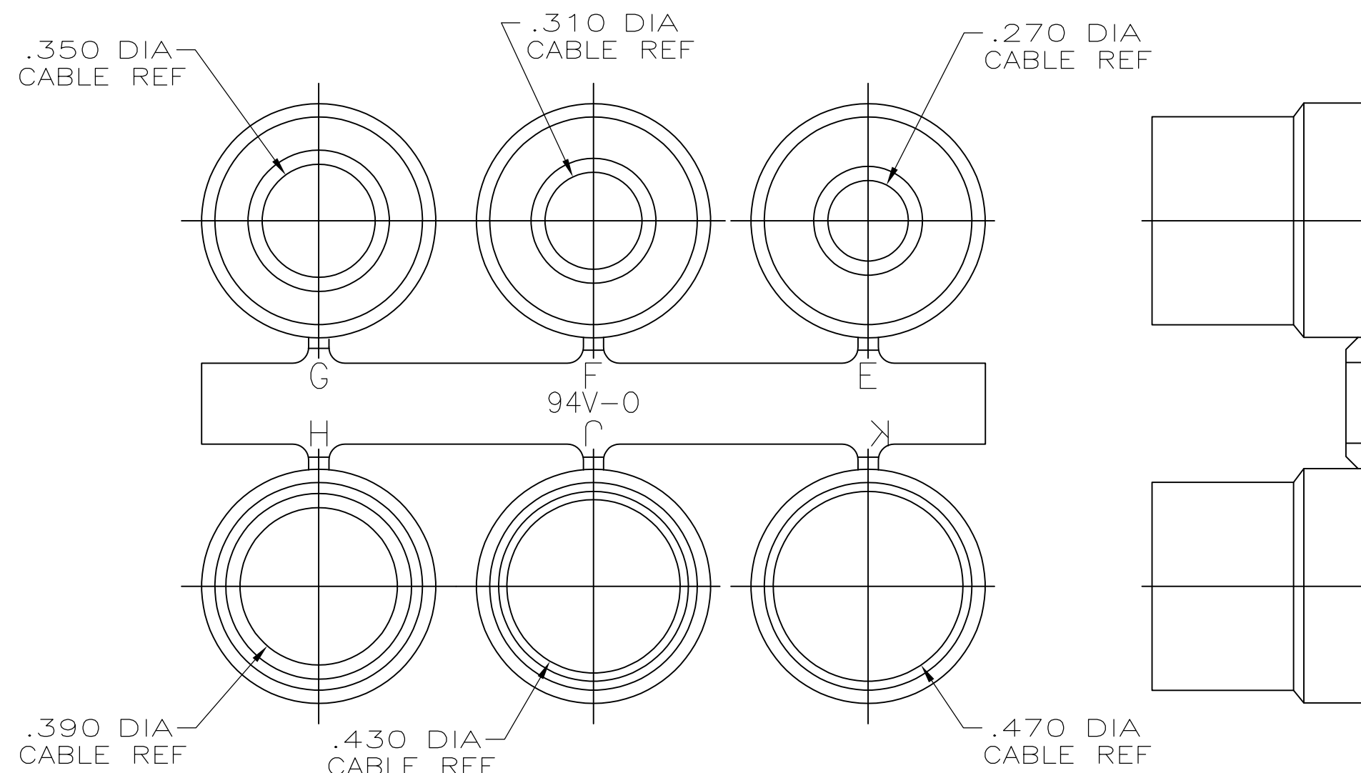
GROMMET ASSORTMENT TYPE 2 SEE TABLE
