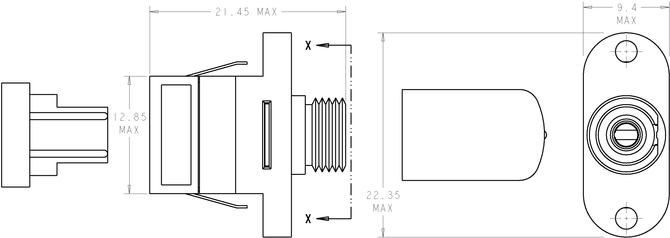
SECTION X-X
