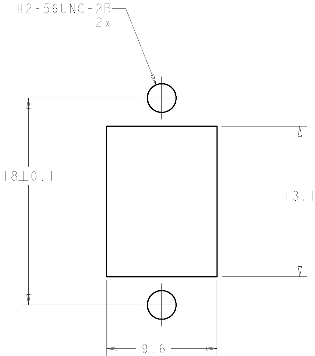
SUGGESTED PANEL CUTOUT MAX PANEL THICKNESS 1.7
