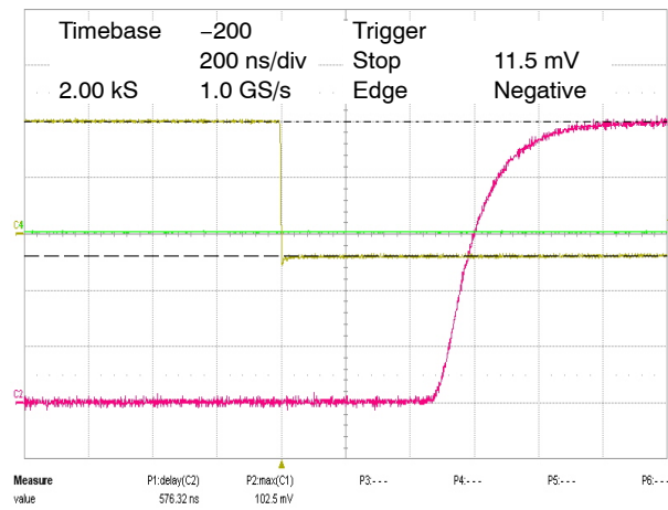
Figure 14. 20 mV Overdrive
